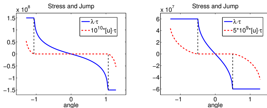
Figure 4: Contact stress in tangential direction and the amplified jump of the displacement in tangential direction for g = 1.5 \times 10^8 (left picture) and g = 0.6 \times 10^8 (right picture).
