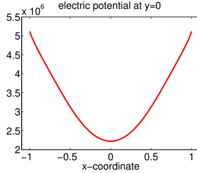
Figure 3: Electric potential at the bottom of \Omega_m .
