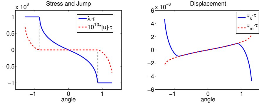
Figure 2: Contact stress \lambda \cdot \tau in tangential direction and the amplified jump of the displacement in tangential direction [u] \cdot \tau (left picture) and the displacements in tangential direction on the slave and the master side u_s \cdot \tau and u_m \cdot \tau on the boundary region \Gamma_3 (right picture).
